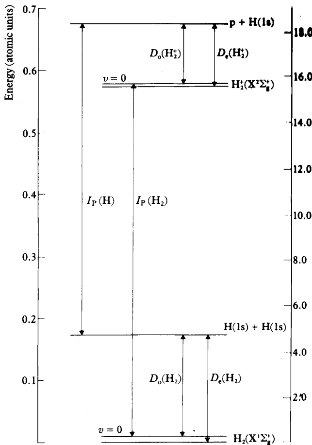
9.14 Relationships between the ground state energies of H_2 , H_2^+ and H. The chemical dissociation energies and spectroscopic dissociation energies denoted by D_0 and D_e , respectively, differ by the zero-point vibrational energy \frac{1}{2}\hbar\omega_0 . The ionisation potentials of the hydrogen atom and hydrogen molecule are denoted by I_P(H) and I_P(H_2) .
